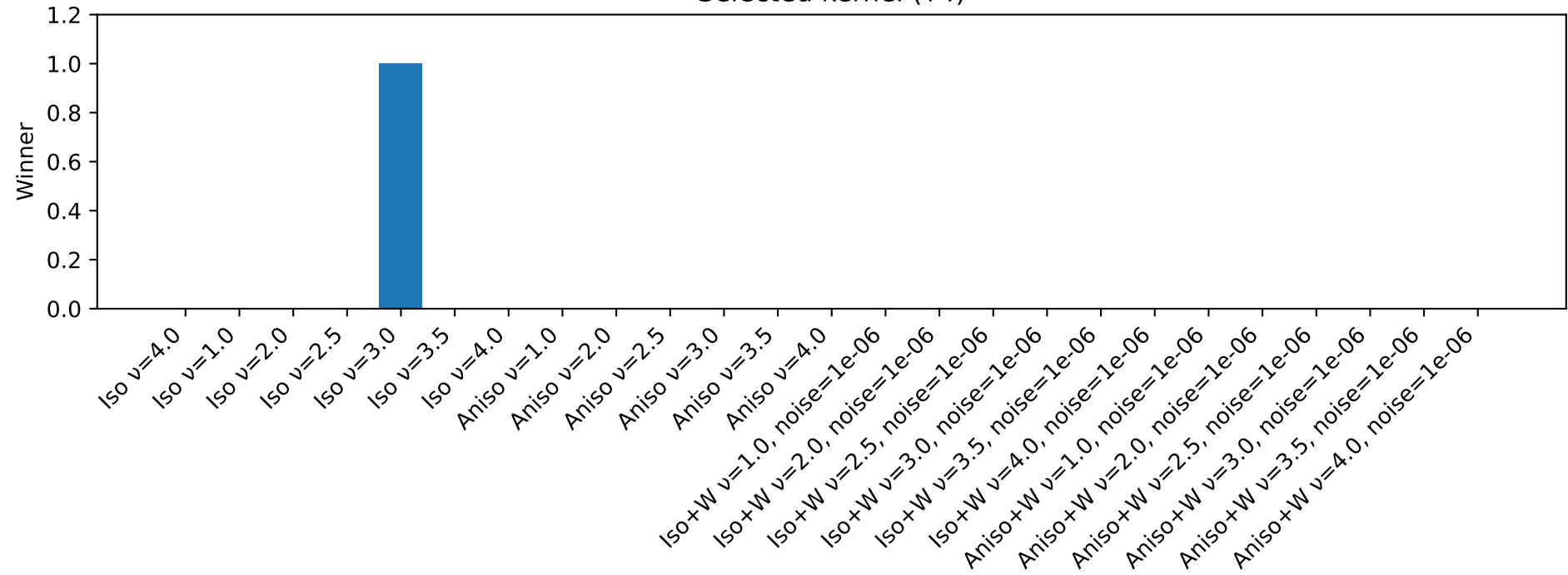
Selected kernel (T4)
