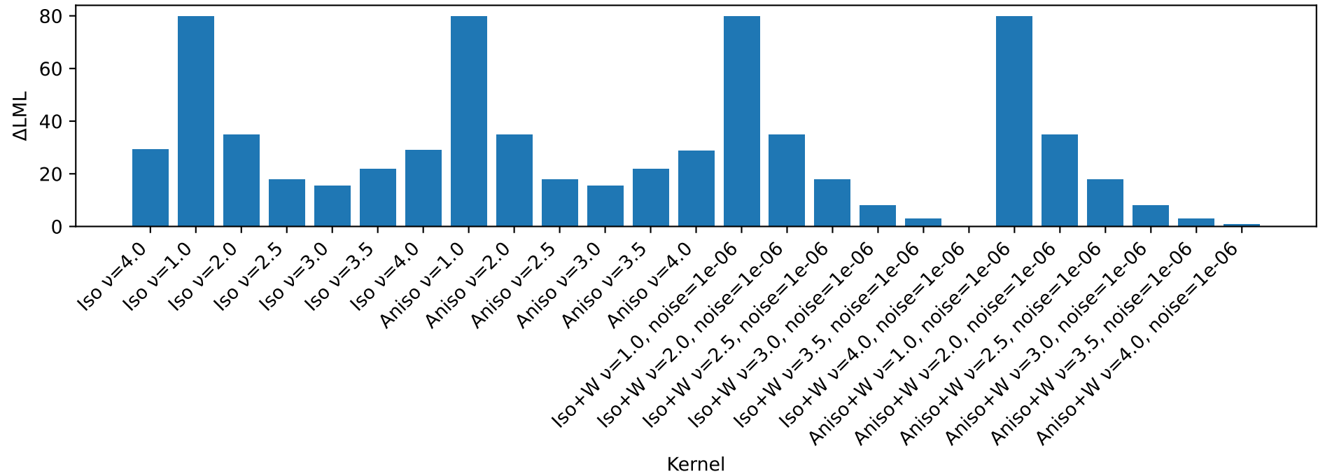
Difference from best LML (T4)
