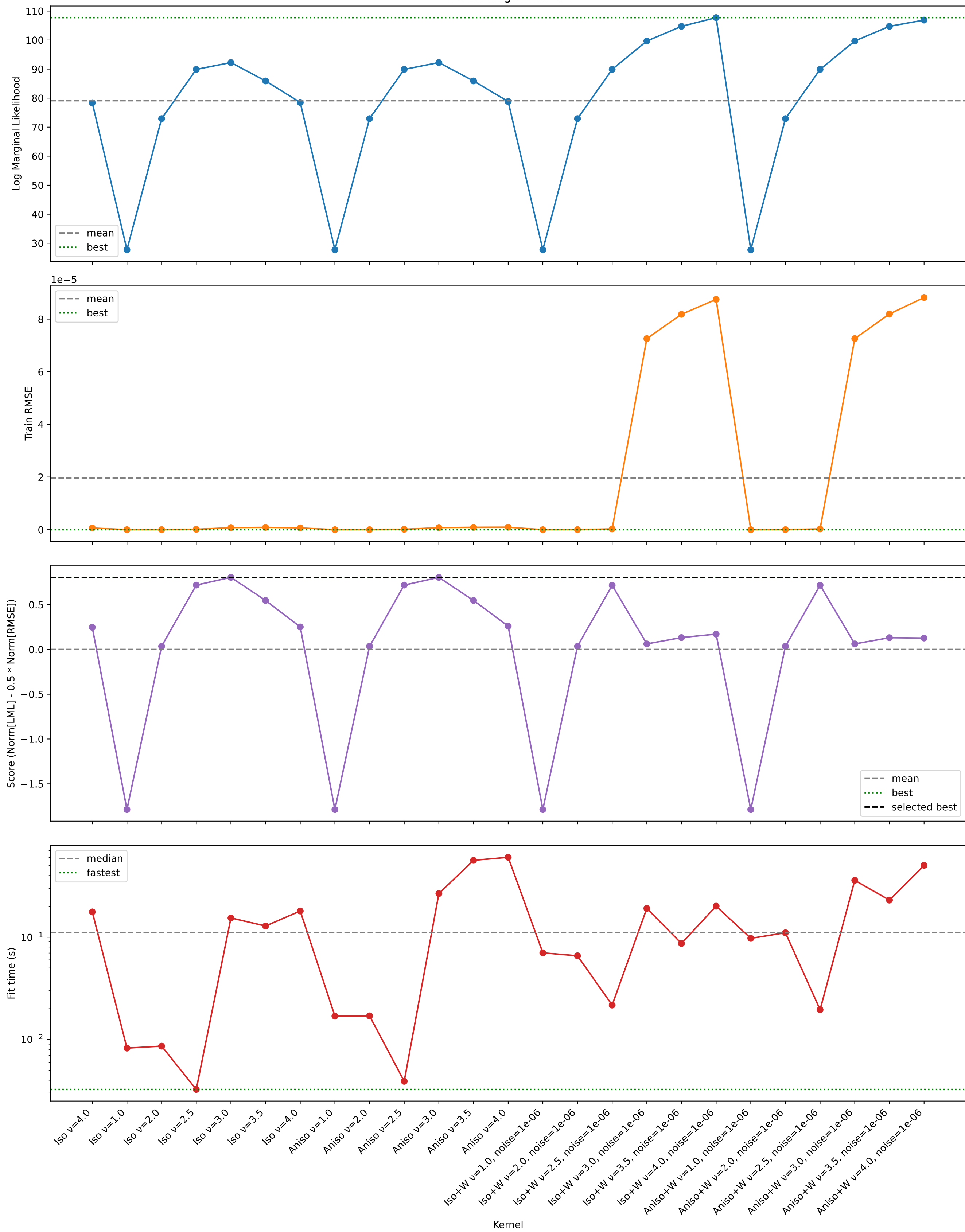
Kernel diagnostics T4
